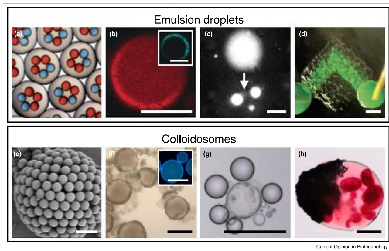
Emulsion-based scaffolds: droplets and colloidosomes. (a) Double-emulsions produced using microfluidic technology, showing blue and red labelled aqueous droplets contained inside oil-in-water droplets. (b) Snapshot of a droplet showing Min protein oscillations at the lipid monolayer. Inset shows the corresponding FtsZ localization in the half where the MinC concentration is low. (c) Interfacial-chemistry-triggered droplet division into multiple daughter droplets. (d) Printed network of droplets, where the green droplets contain membrane pores, enabling ionic current between the electrode-impaled drops. (e) Scanning electron micrograph of a colloidosome. (f) Cross-linked colloidosomes in an aqueous environment. Inset shows the colloidosomes in oil, retaining water-soluble dye. (g) Division of a colloidosome (in the center) into multiple daughters. (h) Artificial phagocytosis of small silica colloids (pink) by a bigger self-propelled Pickering emulsion microdroplet. Panels are adapted as follows: (a) [39]; (b) [41*]; (c) [42]; (d) [43*]; (e) [45]; (f) [46]; (g), [48*]; (h) [49]. Scale bars: 20 \mu\text{m} (b, b inset, c); 200 \mu\text{m} (d, f, g, h); 2 \mu\text{m} (e).
