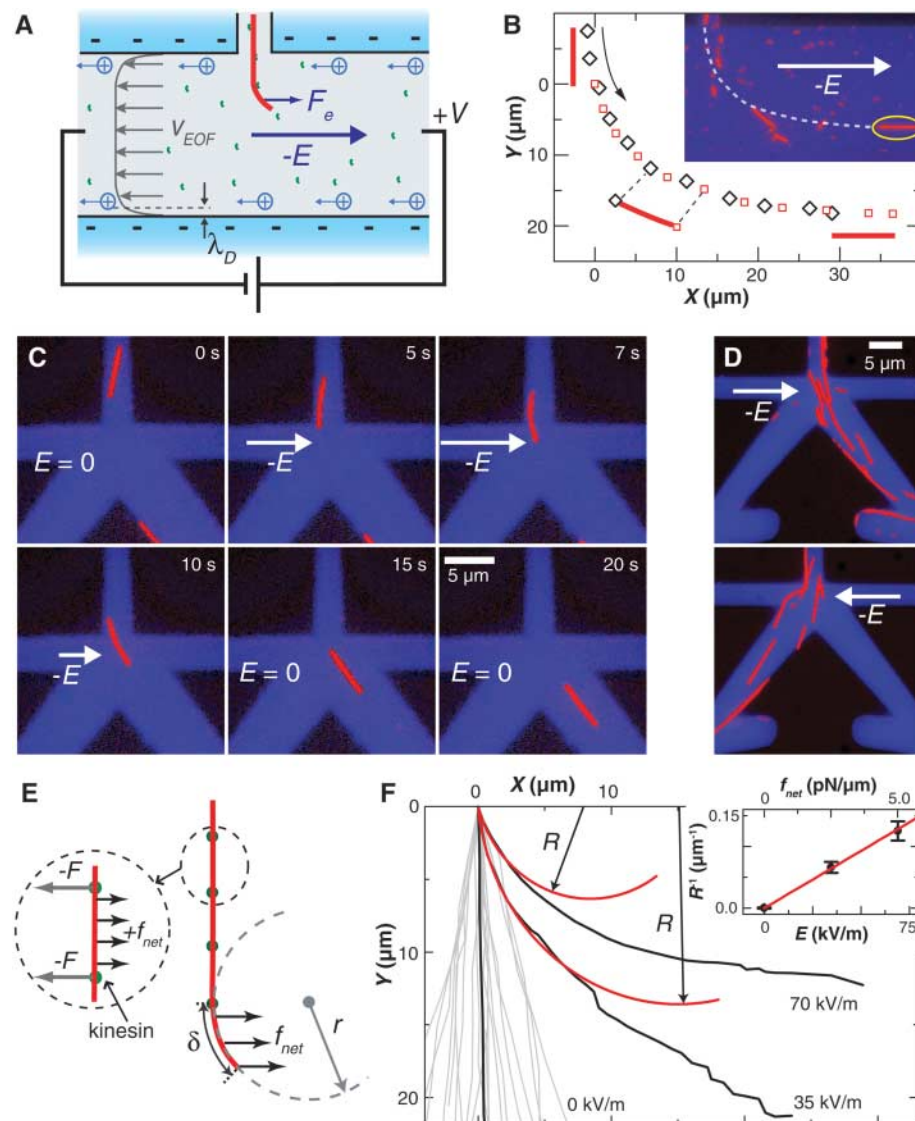
Fig. 2. Bending and steering of microtubules by an electric field. (A) An electric field ( E ) is induced in a horizontal channel perpendicular to the vertical direction of microtubule (red) motion. The electric force on the negatively charged microtubule is along -E , denoted by the blue arrow. Furthermore, the applied electric field will induce motion of the positive ions in the double layer at the channel walls (characteristic thickness \lambda_D ), causing an electro-osmotic flow in the channel. (B) Overlapping coordinates of leading (red symbols) and trailing (black symbols) ends of a microtubule oriented in a field |E| = 50 kV/m. (Inset) The positions trace (dashed) in a fluorescence image. (C) A microtubule entering from the central channel at the top is steered into the right lead of the Y junction by application of a perpendicular electric field that varies in magnitude between 0 and 50 kV/m (indicated by length of arrow). (D) By using magnitude and direction of the electric field, many microtubules are steered to the right (top panel) and left (bottom panel). (E) Bending of a microtubule by a net force. The main part of the microtubule is held fixed by kinesin molecules; only the free leading tip (length \delta ) is subject to a force density f_{net} , which bends it with curvature r^{-1} . (F) Measurements of the average trajectories that microtubules travel under three different applied fields E_x . Black traces represent averages of many individual paths. Gray lines are the individual trajectories at |E| = 0 . At |E| \neq 0 , the spread in the individual trajectories is similar, but they are not shown for clarity. Initial curvatures of the trajectories are denoted by red circles. (Inset) The linear relation between electric field strength |E| and curvature R^{-1} . The values of f_{net} were calculated from E (see text).
