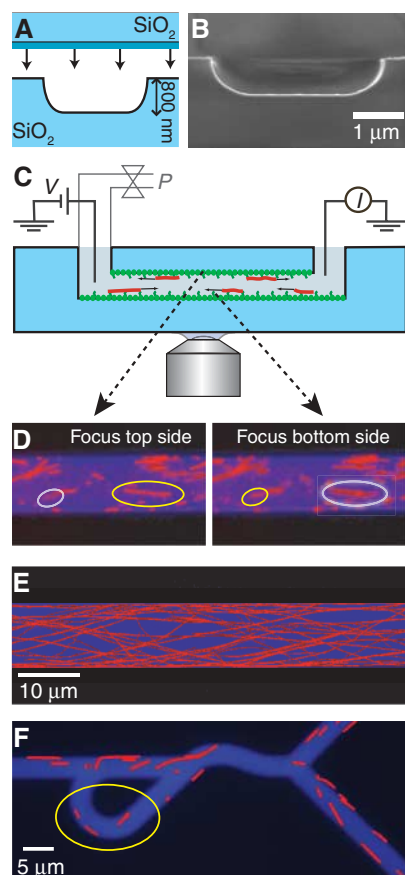
Fig. 1. Enclosed submicron channels allow for full confinement of microtubules. (A) E-beam lithography and wet etching create 800-nm-deep trenches in SiO 2 substrates. A coverslip coated with a sodium-silicate solution (dark blue) seals the channel after annealing. (B) Scanning electron microscopy image of a cross section of a nanochannel. (C) Schematic cross section along a channel. Kinesin motor proteins (green) and microtubule filaments (red) are added to the channels by a pressure-driven flow. Electric fields can be induced in the channels by applying a potential difference between the reservoirs. (D) Fluorescence microscopy shows that microtubules (red) move on both sides of the channels (blue). Yellow ovals indicate microtubules in the focal plane; white ones denote microtubules just out of focus. (E) Traces of several microtubules moving through a confined channel. The figure is an overlay of microtubule traces traversing the image during a period of 7 min. No microtubules are observed outside of the tracks. (F) More complex geometries, such as the bend in a rectifying geometry, could also be well coated with kinesin molecules and could support microtubule motility.
