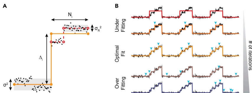
Figure 2. Global arrangement of the AutoStepfinder algorithm
